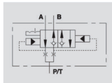
Hydraulic Symbol
