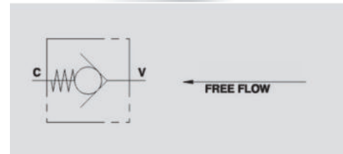
Hydraulic Symbol
