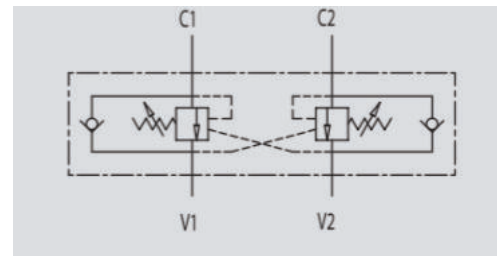
Hydraulic Symbol
