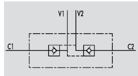
Hydraulic Symbol
