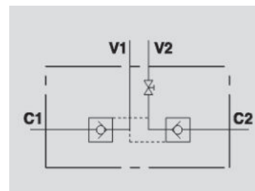
Hydraulic Symbol
