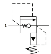
Hydraulic Symbol
