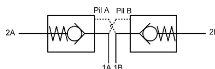
Hydraulic Symbol
