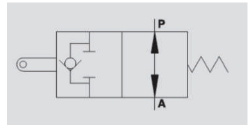
Hydraulic Symbol
