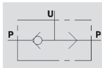
Hydraulic Symbol
