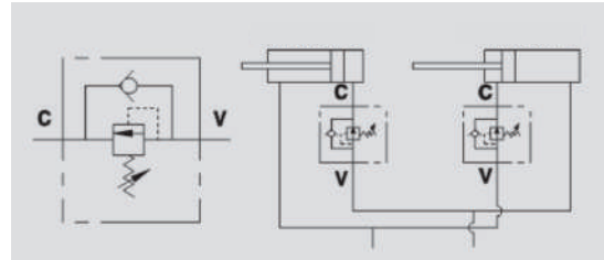
Hydraulic symbol
